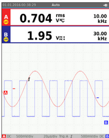
Fluke Connect-and-View™ triggering with Auto Reading function using Fluke IntelliSet™ technology gives you quick access to the data you need.
