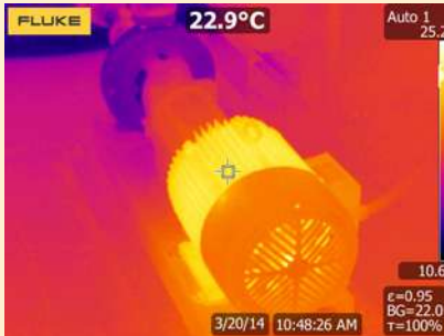
Combo: This heat pattern indicates an operational motor.
