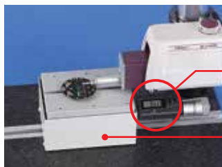
Digimatic micrometer head Amount of micrometer head adjustment required Leveling table (DAT) (Option)
