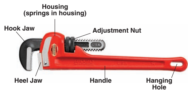
Figure 2 – Wrench Parts
