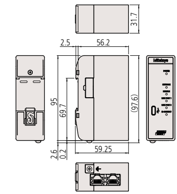
Interface unit PROFINET
