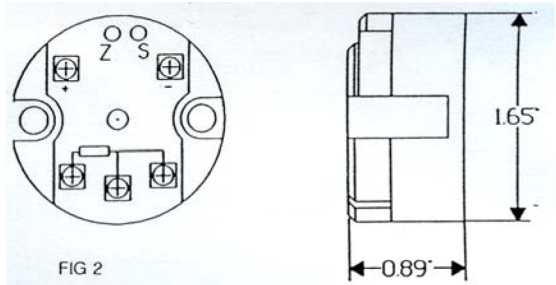
FIG 2 Mounting holes : 2 hole 0.22. 1.3 centers Center-hole sensor wire entry : 0.16 diameter
