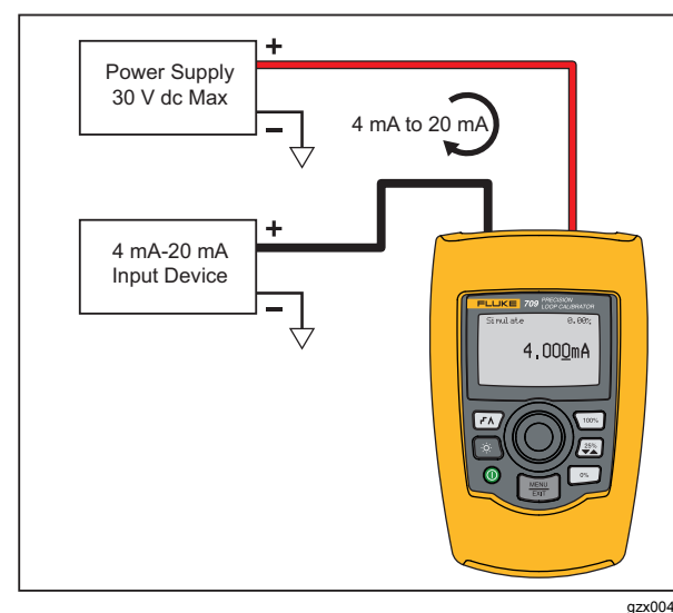
Figure 5. mA Simulate Connections
