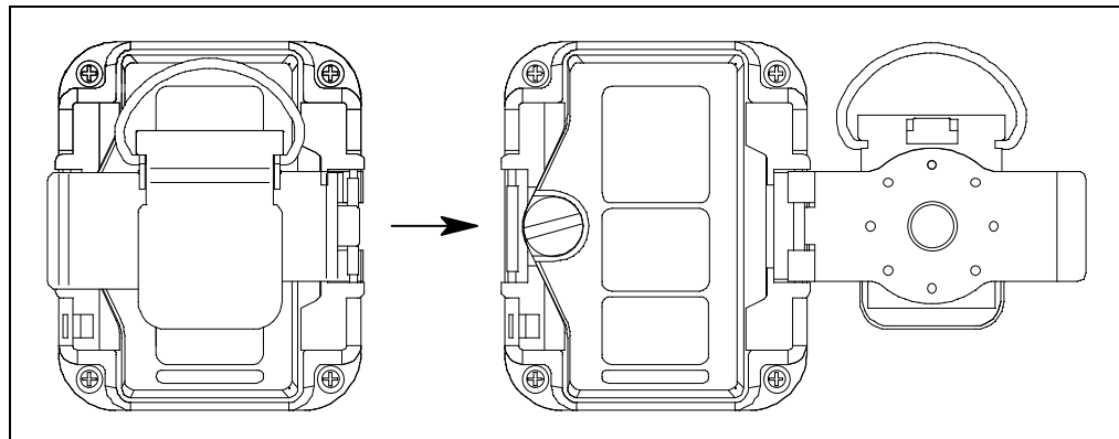
Figure 7: Releasing the Alligator or Belt Clip
