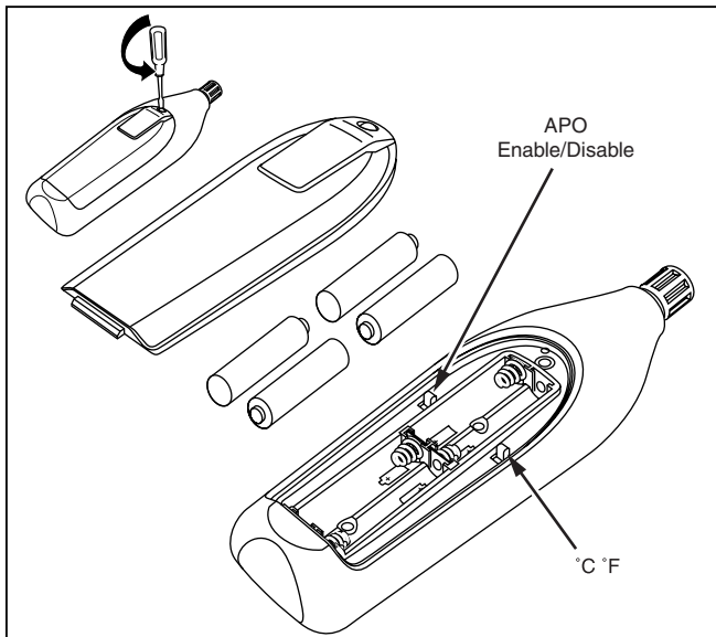
Figure 1. Battery Compartment
