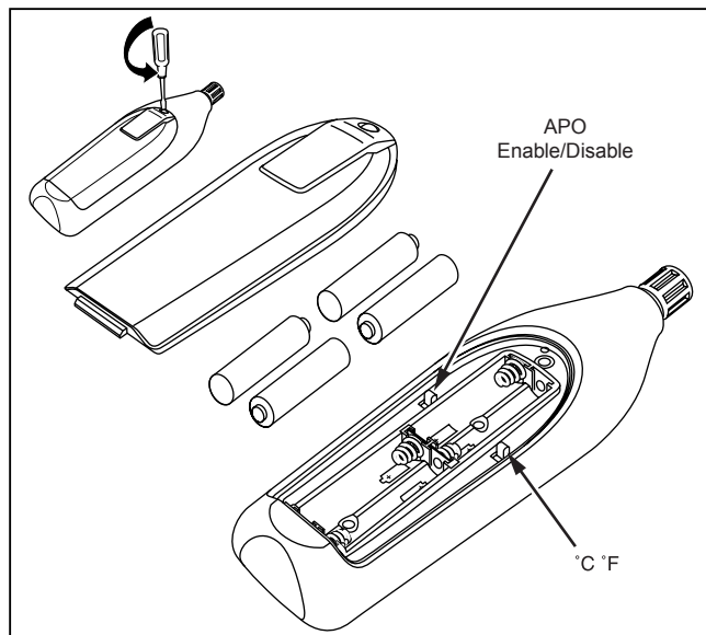
Figure 1. Battery Compartment
