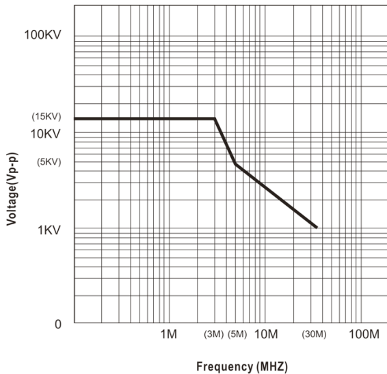
Figure 2. CT4076 Derating Curve
