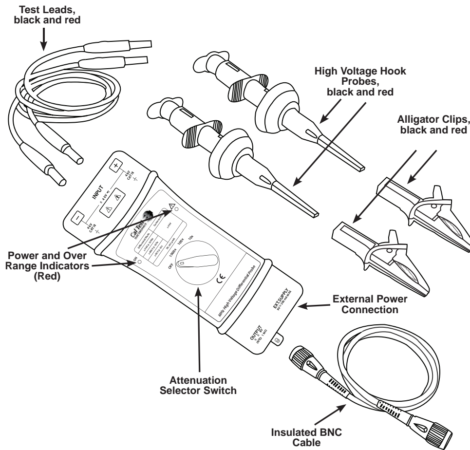
Figure 1 Front Panel Features
