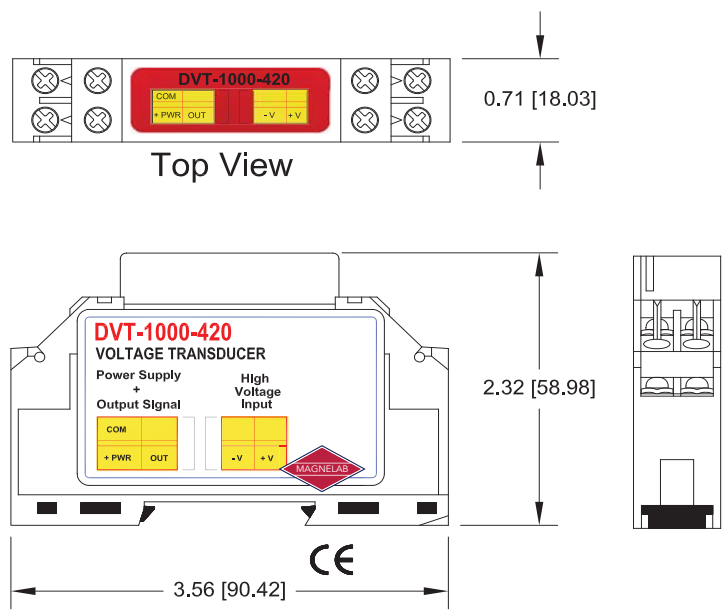
Dimensions are in inches and Millimeters
