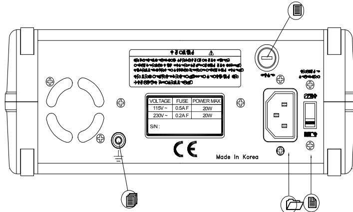
FIG 2-2. REAR PANEL(8105,8110)
