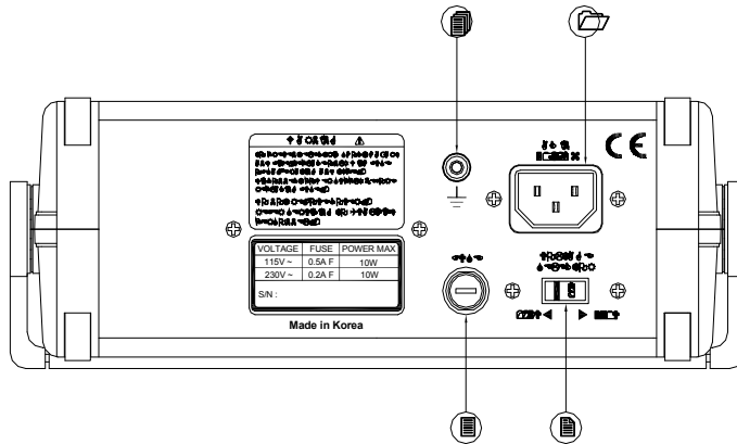
FIG 2-1. REAR PANEL(8102,8103)
