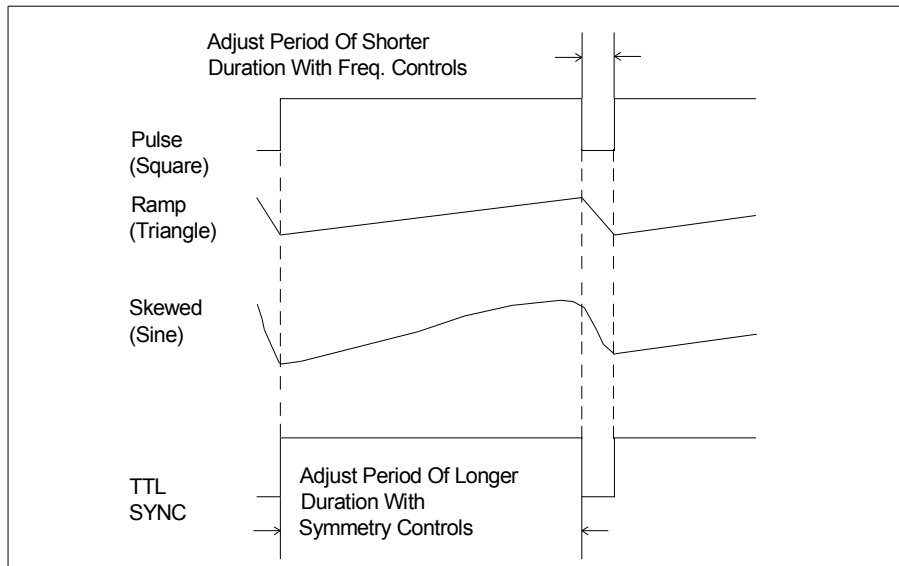
FIG 5. PULSE, RAMP, AND SKEWED SINE WAVE GENERATION
