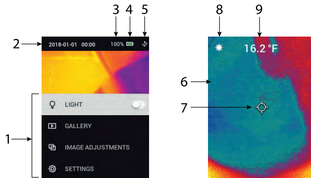
Figure 3.2 IRC130 Displays
