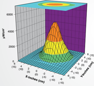
Surface Contour Profile at 15 in (38 cm)
