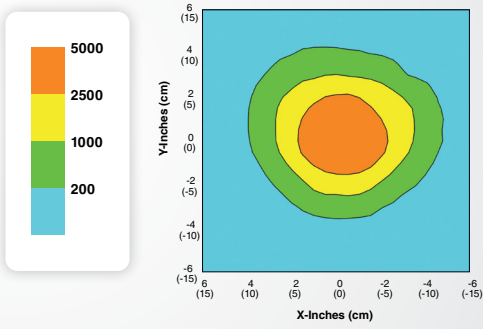
Top Intensity Profile at 15 in (38 cm)
