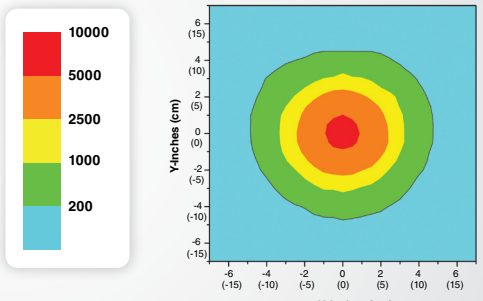
Top Intensity Profile at 15 in (38 cm)
